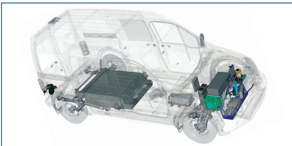
Azure Dynamics will integrate its Force Drive™ battery electric drivetrain in the Ford Transit Connect Electric.
